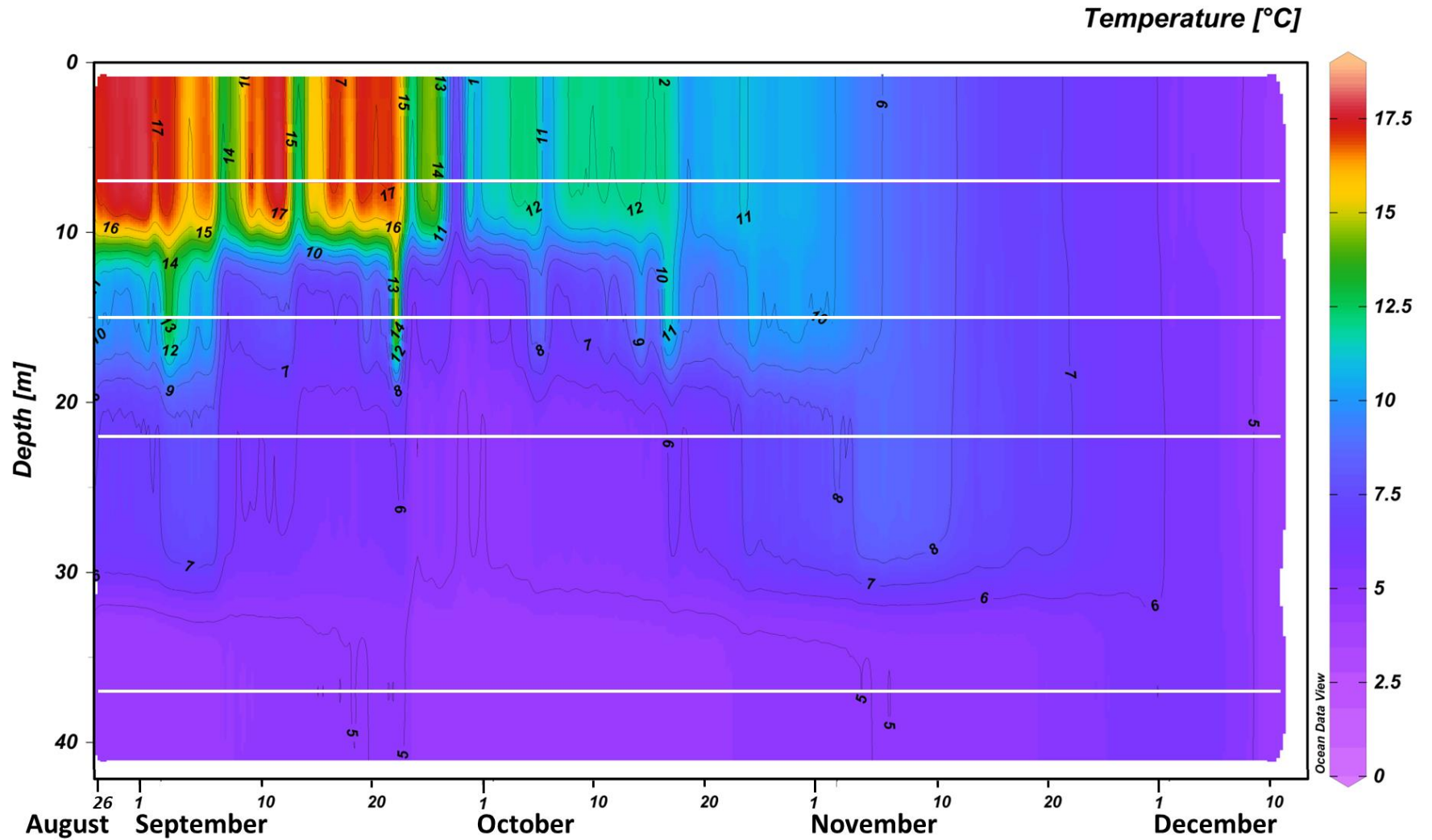
Figure B1-6.4-2 Temperature Model at T1 in Argentina Harbour from Aug 26 and Dec 10, 2023.
