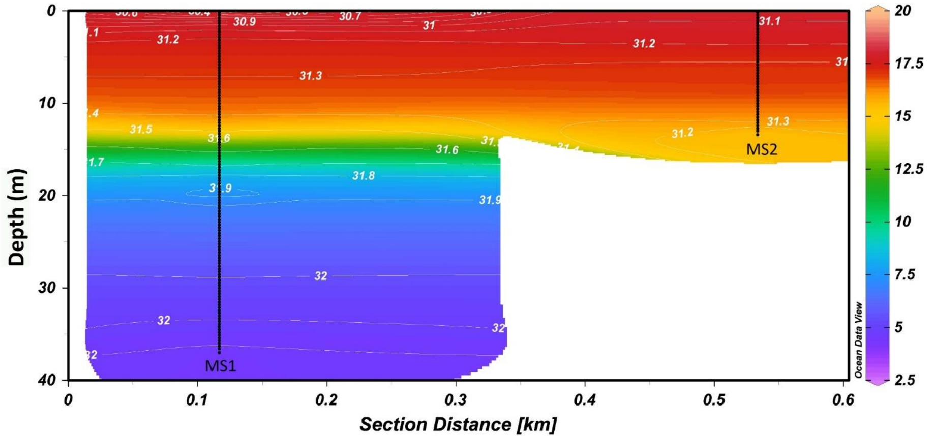
Figure B1-6.3-2 Temperature and Salinity Model of the Two Marine Stations, August 26, 2023.
