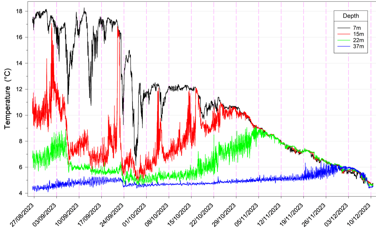
Figure B1-6.4-1 Temperature Profile at T1 in Argentinia Harbour from Aug 26 to Dec 10, 2023.
