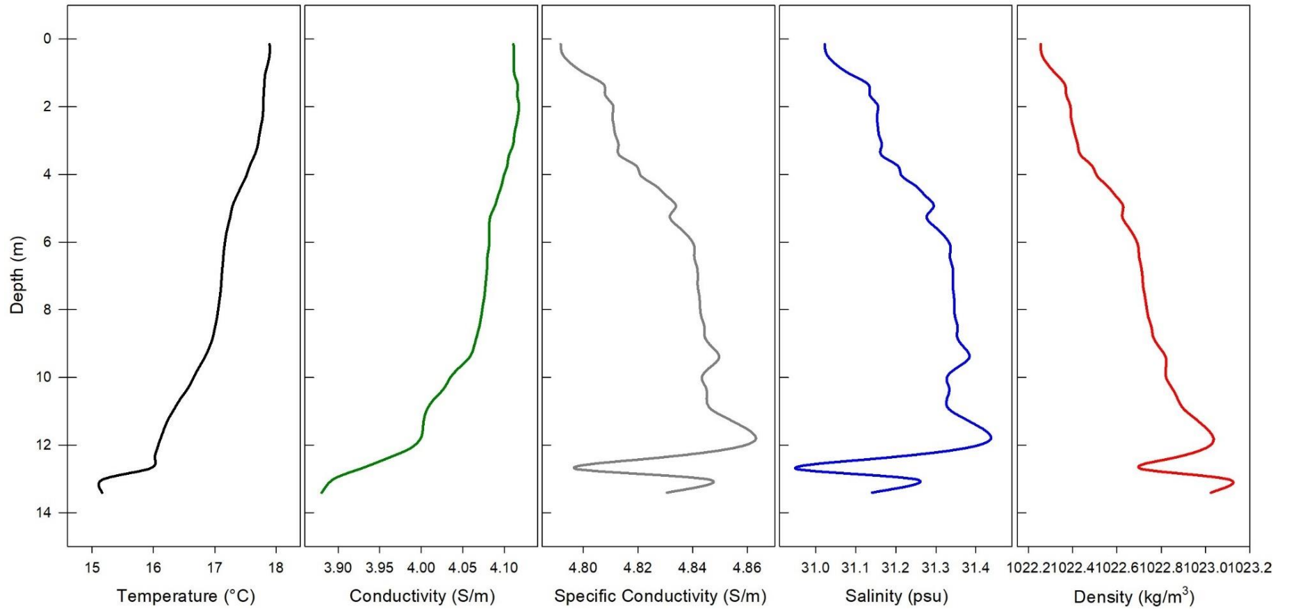
Figure B1-6.2.3-1 Marine Station 2 CTD Profile, Aug 26, 2023.
