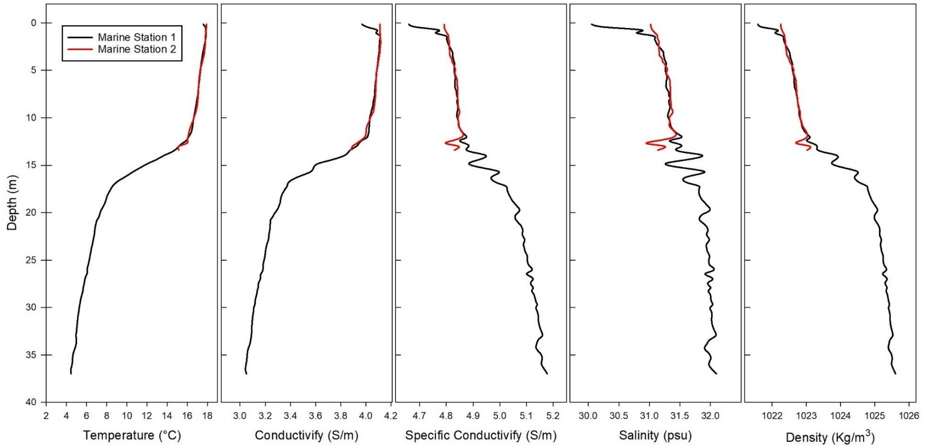
Figure B1-6.3-1 Combined Marine Station CTD Profiles, Aug 26, 2023.
