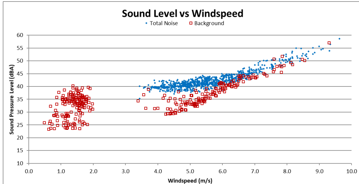
Figure 3: V6202 – Measured Sound Levels for Turbine ON and Background vs Wind Speed
