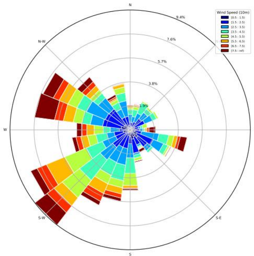
Figure 2: Measured wind rose for R3214 for the Phase 2 I-audit campaign 7
