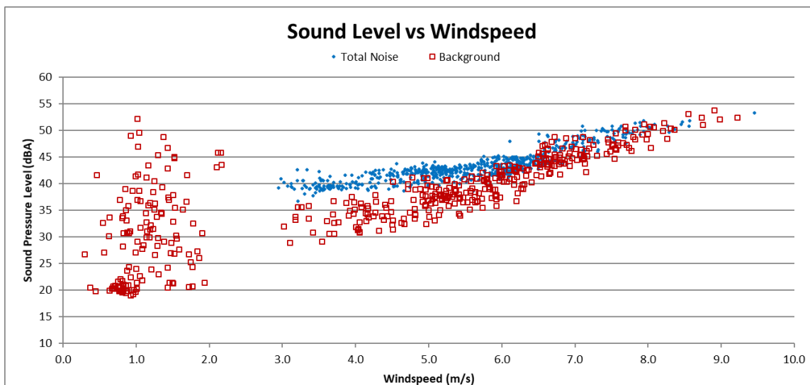
Figure 3: R3214 - Measured Sound Levels for Turbine ON and Background vs Wind Speed
