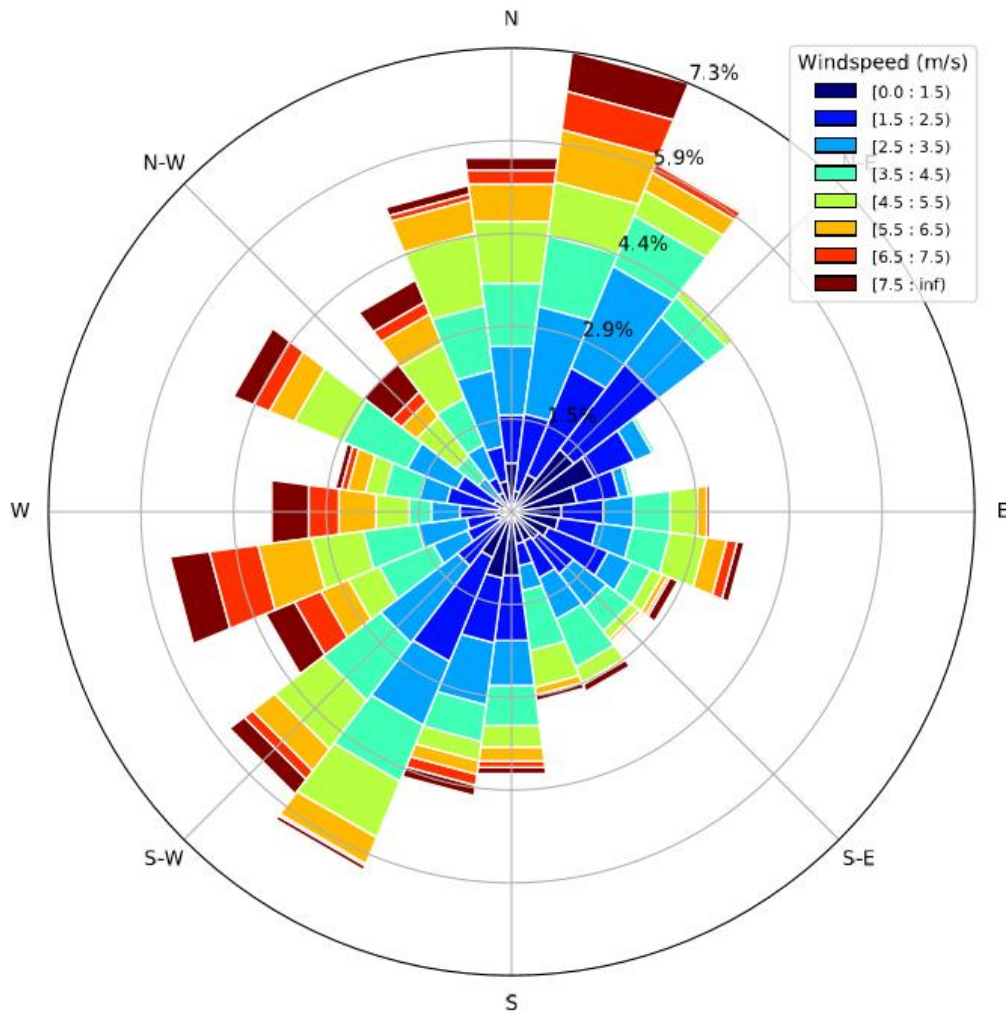
Figure 2: Measured wind rose for R3099 for the Phase 1 I-audit campaign 6
