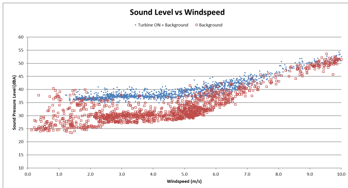
Figure 4: R3408- Measured Crosswind Sound Levels for Turbine ON and Background vs Wind Speed
